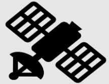
Inferences
